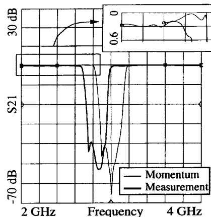
Fig. 5. Measurement at 35 K versus Momentum simulation.
