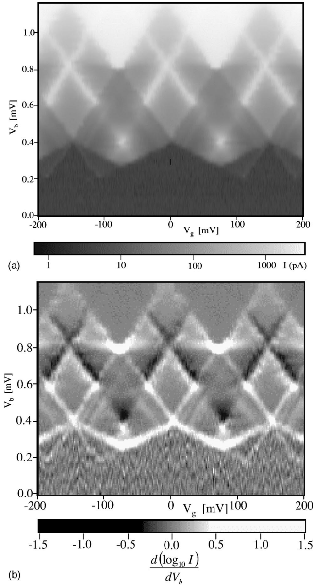
FIG. 4. (a) The logarithm of the current through a superconducting SET transistor is plotted as a function of the bias voltage and the gate voltage. (b) The same derivative of the same data shown in (a).
